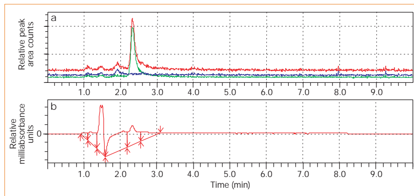
Figure 2 Chromatographic analysis of residue from Maya cooking vessels. a , Mass-spectrometry chromatogram of dry extract from vessel 13. Red, total-ion chromatogram; green, selected-ion monitoring (SIM) at m/z=181 for theobromine; blue, SIM at m/z=195 for caffeine. For the mass spectrum of the peak at 2.6 min, as well as details of methods and standards, see supplementary information. b , Ultraviolet chromatogram of the same extract, showing a peak at 2.6 min, which is consistent with results in a . Dashed lines are integration markers; arrows indicate the starts and ends of peaks. The peak at around 1.5 min is due to the chromatography solvent. The peak for caffeine is not evident as its concentration in cocoa is about 10 times lower than that of theobromine.
